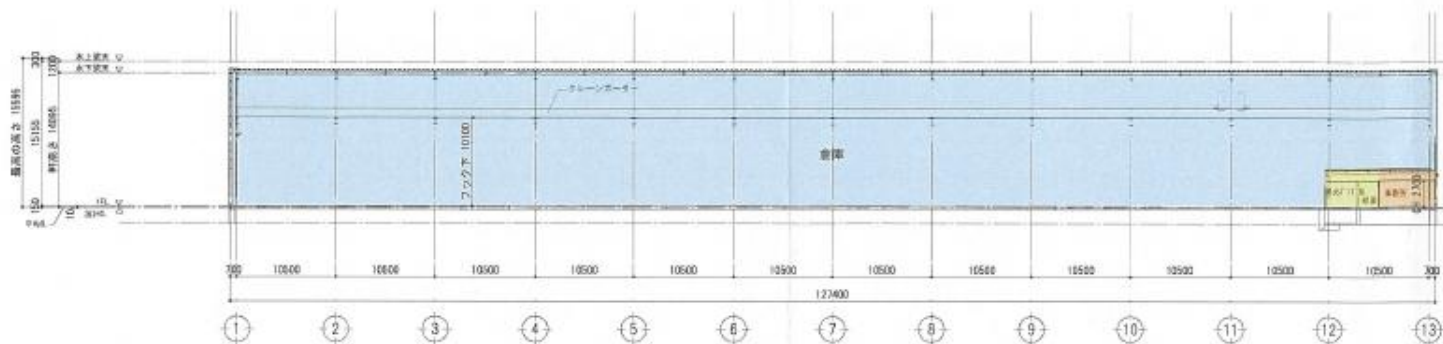
断面図_B
